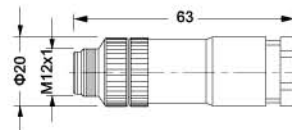
现场接线 / 可接 2 根电缆 Field-wireable / Can receive 2 cables can receive 2 cables
