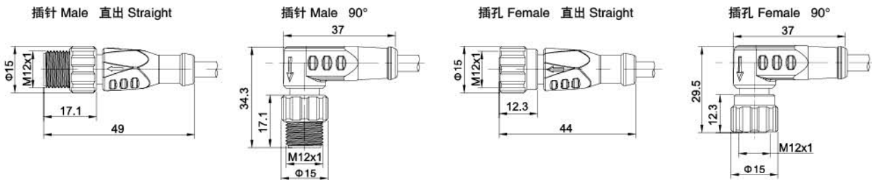
单端预铸线束 With open ended wires
